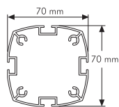
4 Channel Profile
