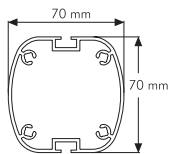
2 Channel Profile
